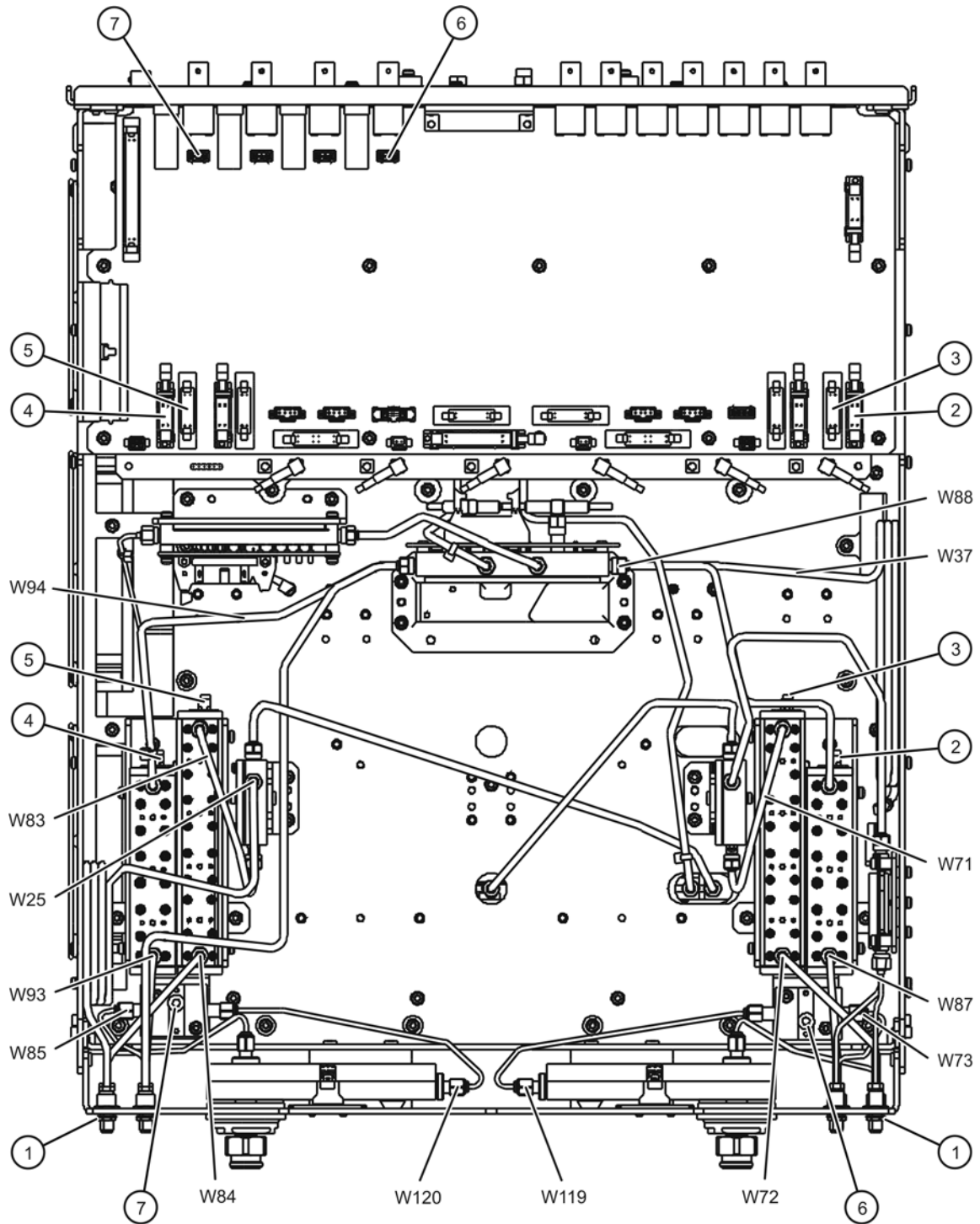
Figure 7 New Cable Installation
